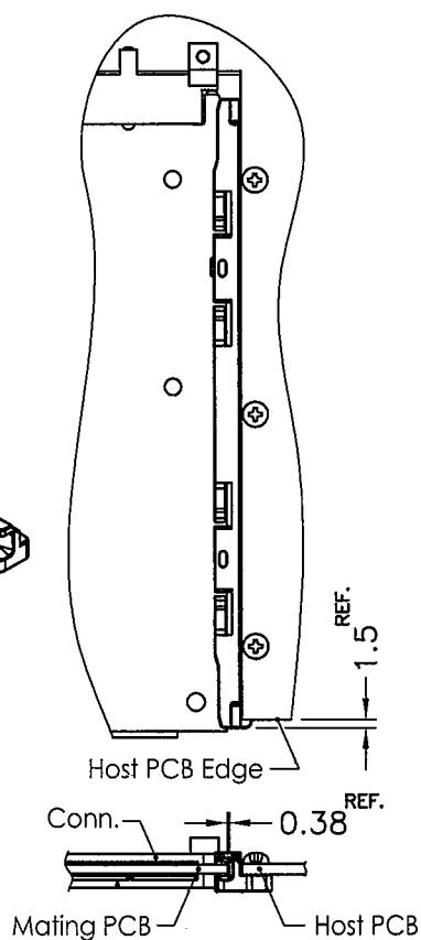
Middle Board Assembly Diagram
