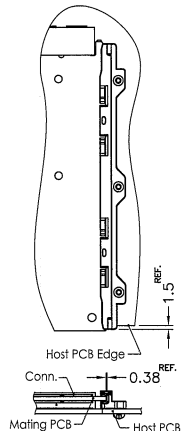
Above Board Assembly Diagram
